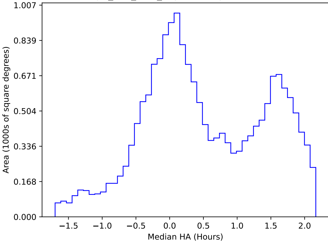
telescope_jerk_v3.5_10yrs WFD g band: Median HA
