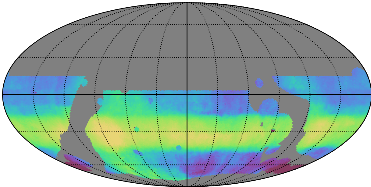
telescope_jerk_v3.5_10yrs WFD all bands: Median HA
