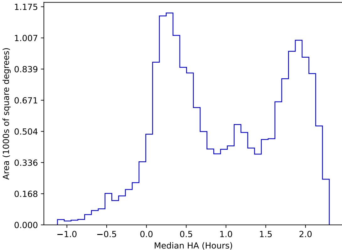
telescope_jerk_v3.5_10yrs WFD all bands: Median HA
