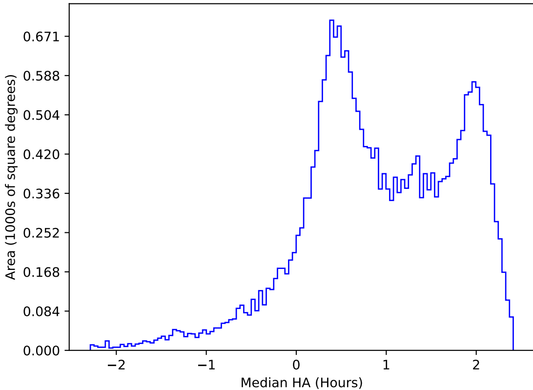
telescope_jerk_v3.5_10yrs All sky z band: Median HA
