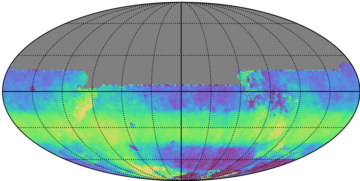
telescope_jerk_v3.5_10yrs All sky y band: Median HA
