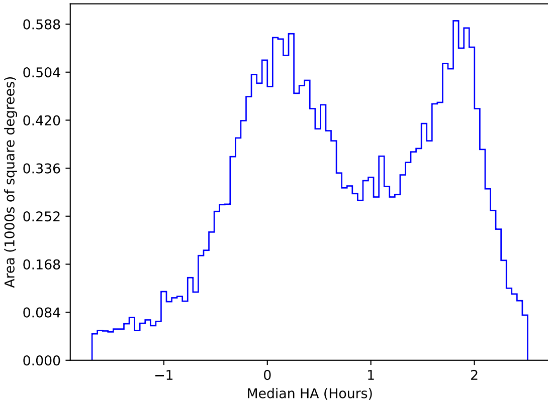
telescope_jerk_v3.5_10yrs All sky u band: Median HA
