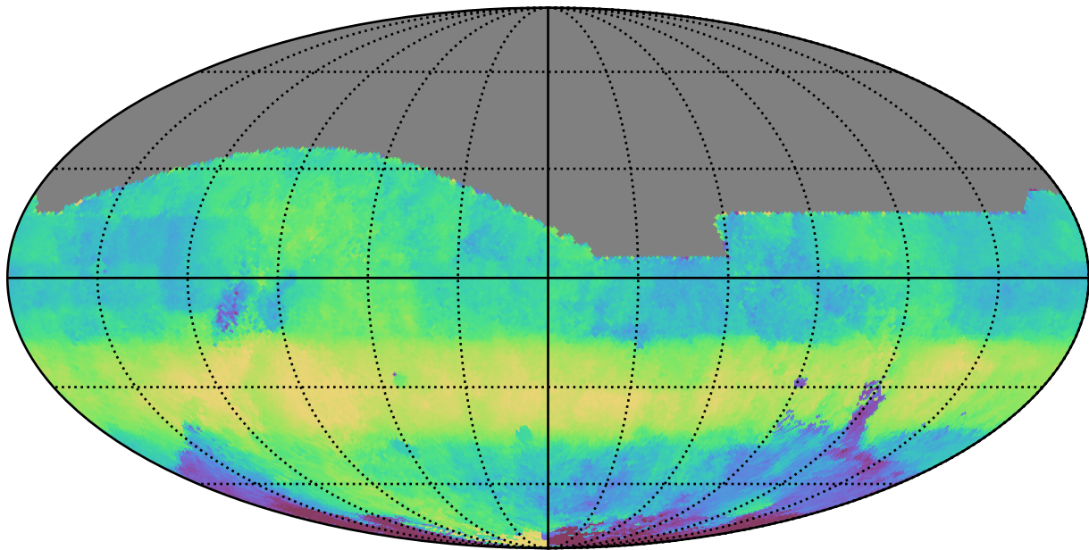
telescope_jerk_v3.5_10yrs All sky r band: Median HA
