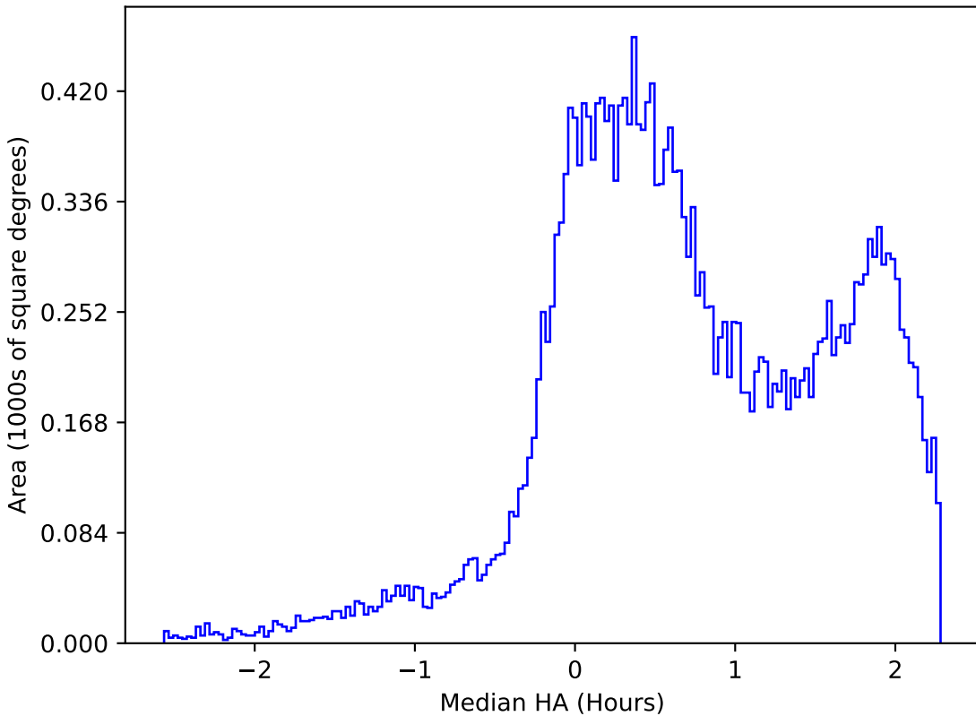
telescope_jerk_v3.5_10yrs All sky r band: Median HA
