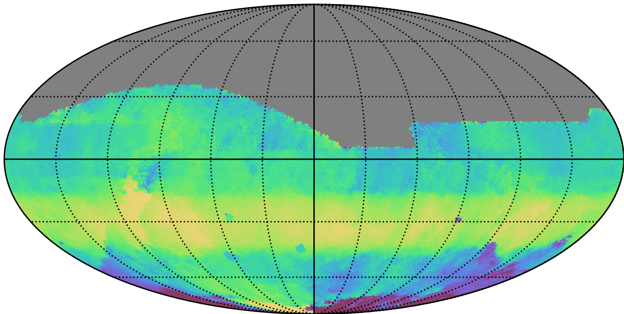
telescope_jerk_v3.5_10yrs All sky i band: Median HA
