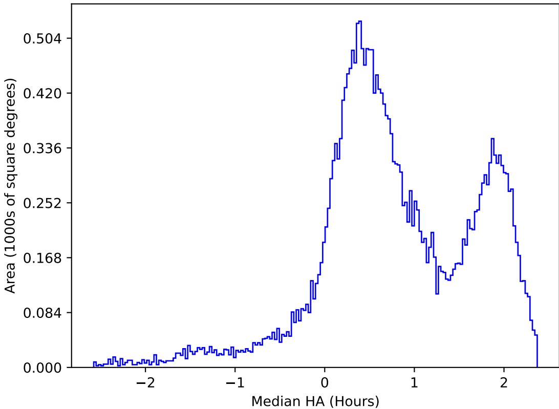
telescope_jerk_v3.5_10yrs All sky i band: Median HA
