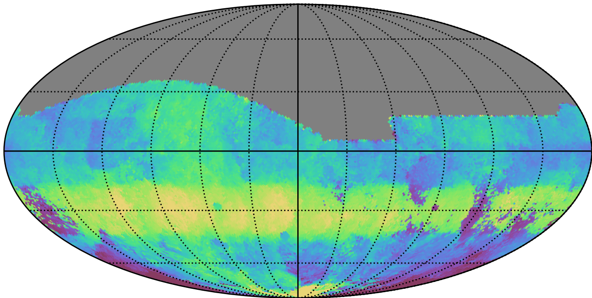
telescope_jerk_v3.5_10yrs All sky g band: Median HA
