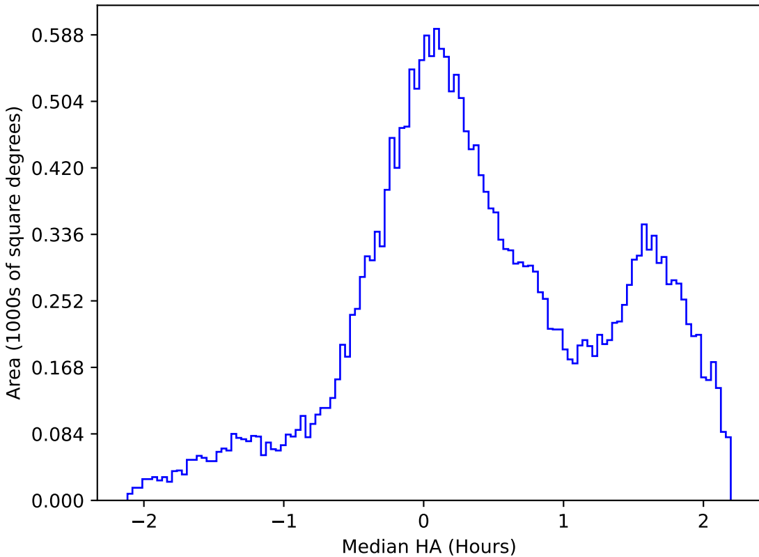
telescope_jerk_v3.5_10yrs All sky g band: Median HA
