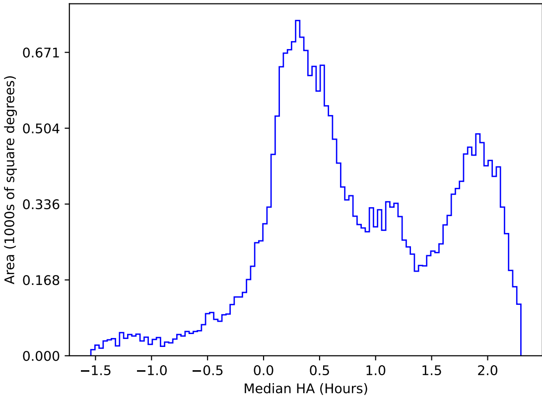
telescope_jerk_v3.5_10yrs All sky all bands: Median HA
