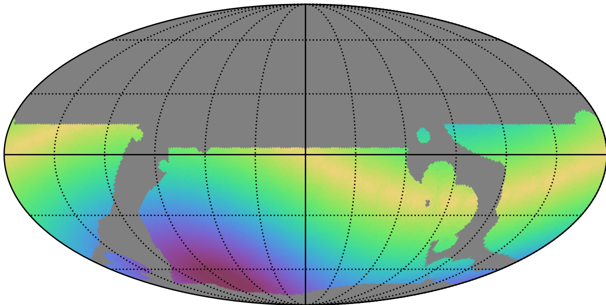
telescope_jerk_v3.5_10yrs WFD y band: Max solarElong
