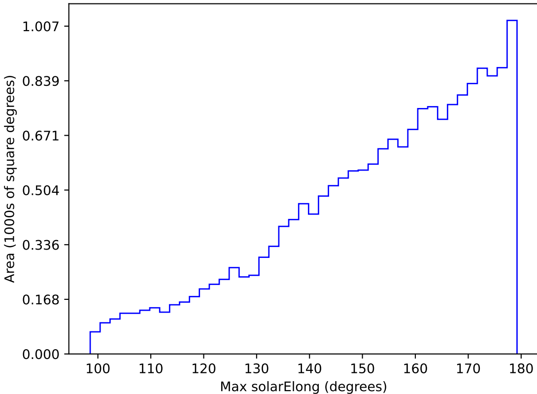
telescope_jerk_v3.5_10yrs WFD y band: Max solarElong
