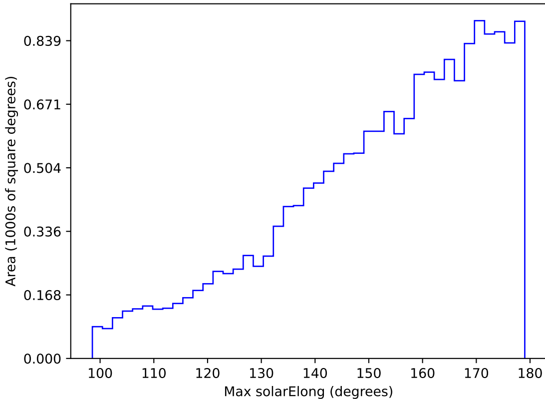
telescope_jerk_v3.5_10yrs WFD u band: Max solarElong
