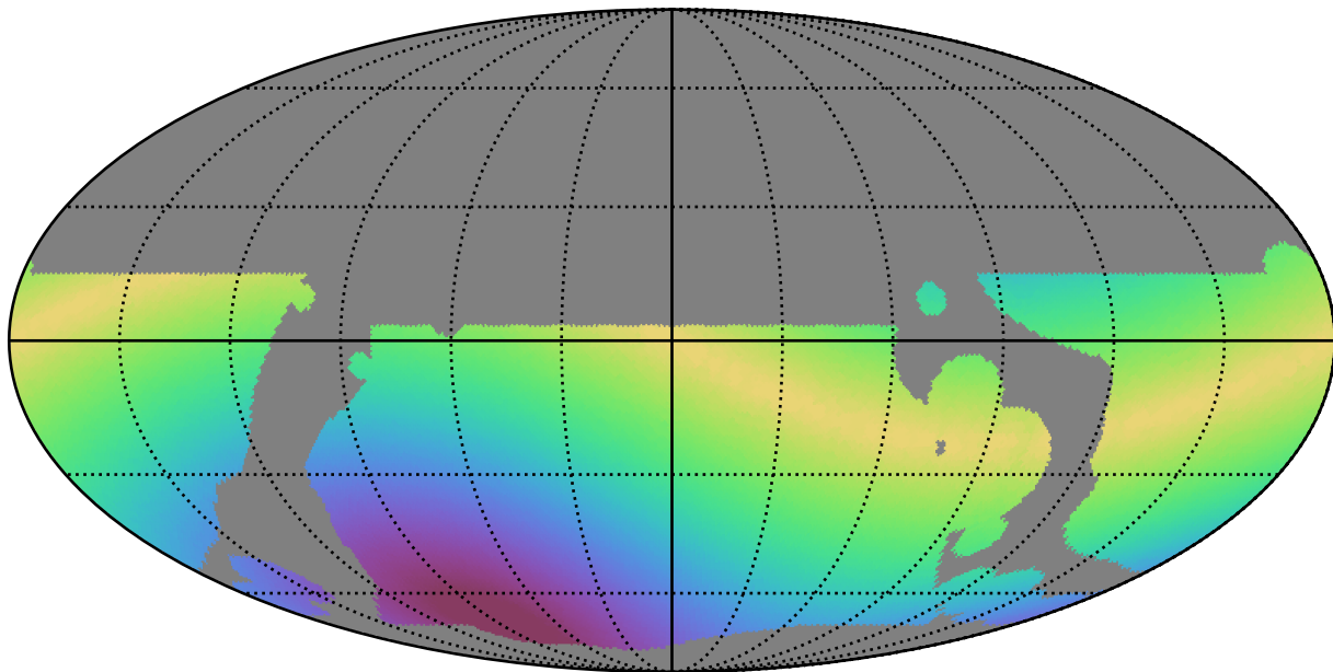
telescope_jerk_v3.5_10yrs WFD r band: Max solarElong
