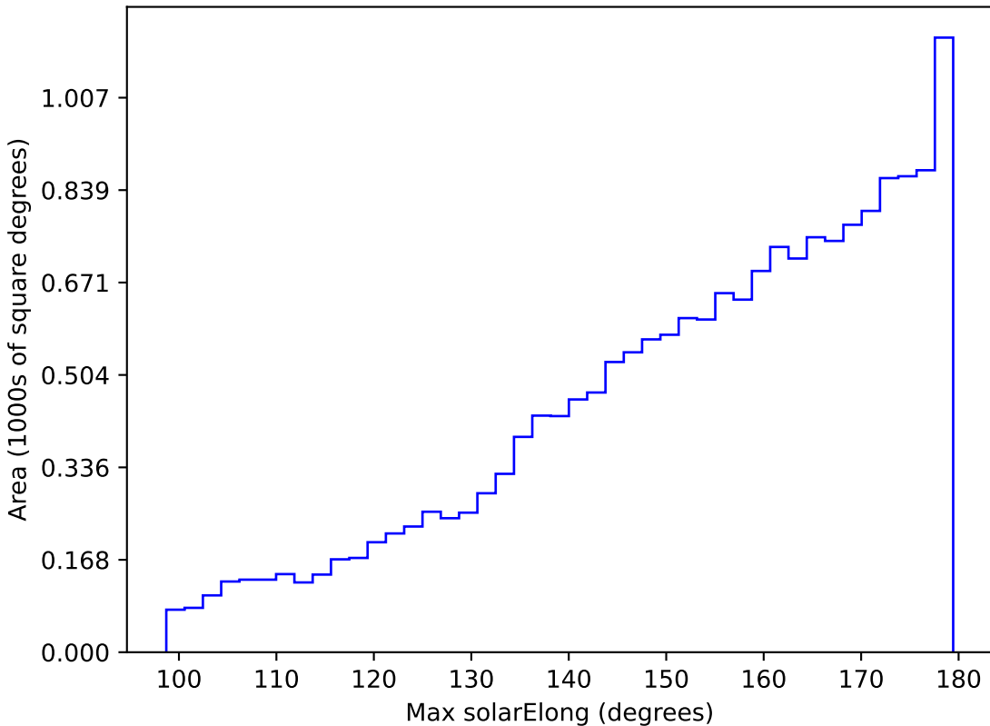
telescope_jerk_v3.5_10yrs WFD r band: Max solarElong
