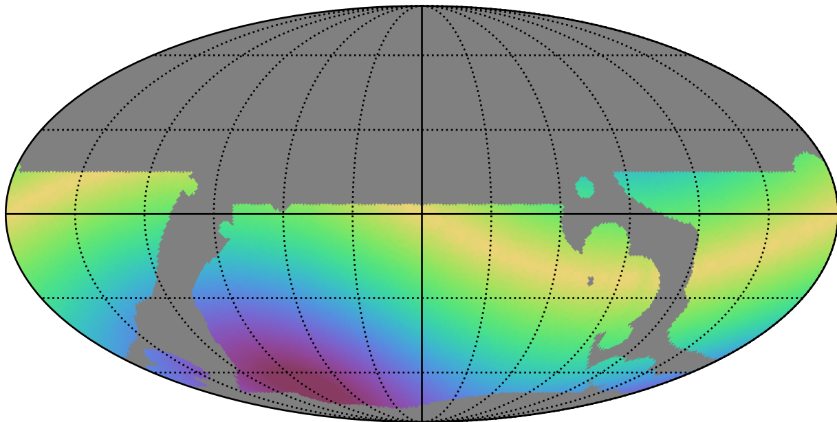
telescope_jerk_v3.5_10yrs WFD i band: Max solarElong
