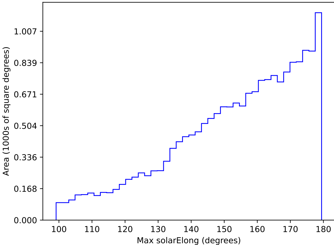
telescope_jerk_v3.5_10yrs WFD i band: Max solarElong
