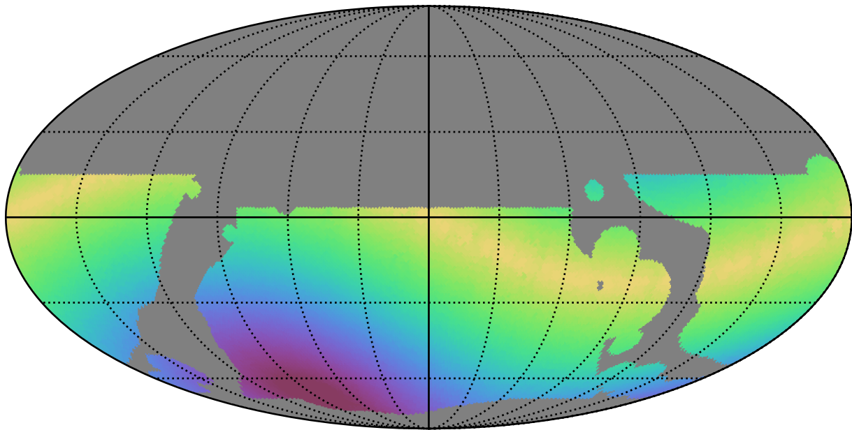
telescope_jerk_v3.5_10yrs WFD g band: Max solarElong
