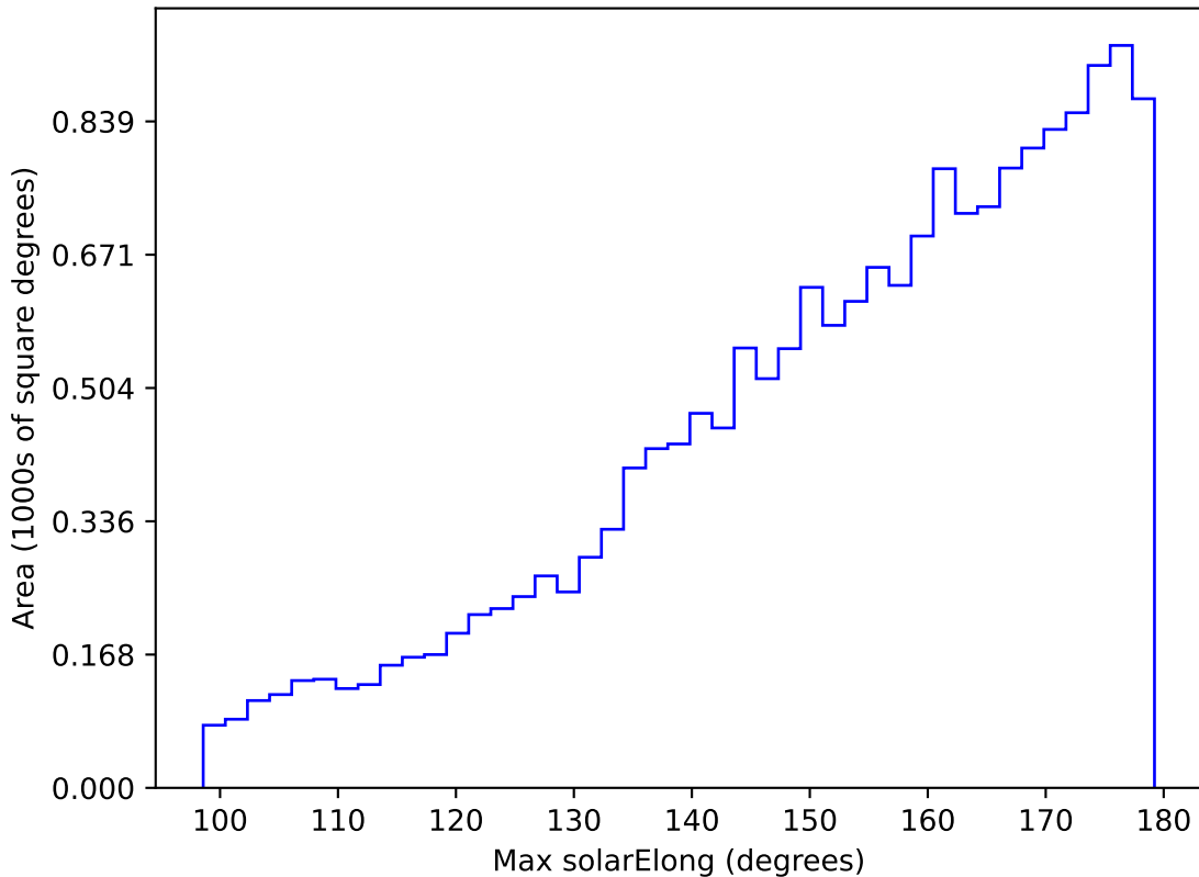
telescope_jerk_v3.5_10yrs WFD g band: Max solarElong
