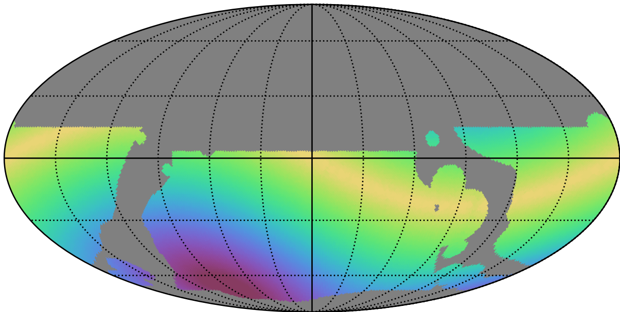
telescope_jerk_v3.5_10yrs WFD all bands: Max solarElong
