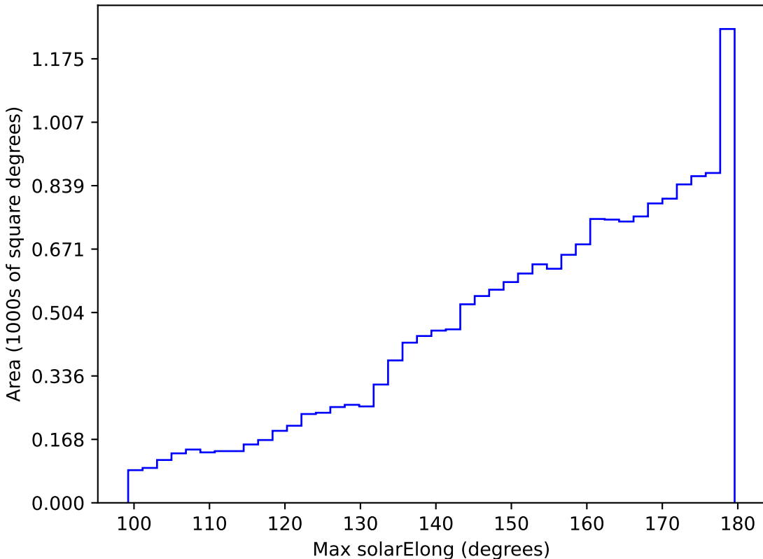
telescope_jerk_v3.5_10yrs WFD all bands: Max solarElong
