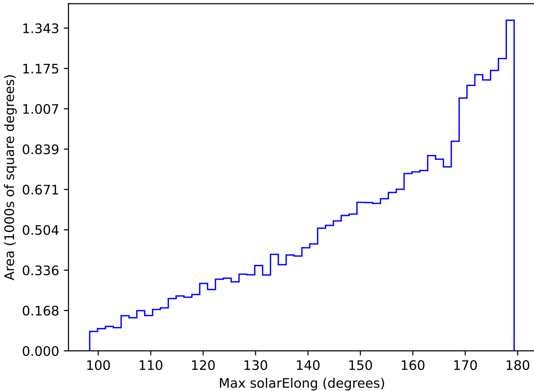
telescope_jerk_v3.5_10yrs All sky z band: Max solarElong
