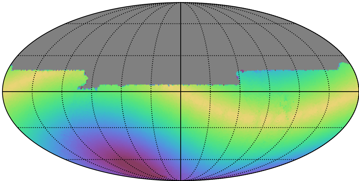
telescope_jerk_v3.5_10yrs All sky y band: Max solarElong
