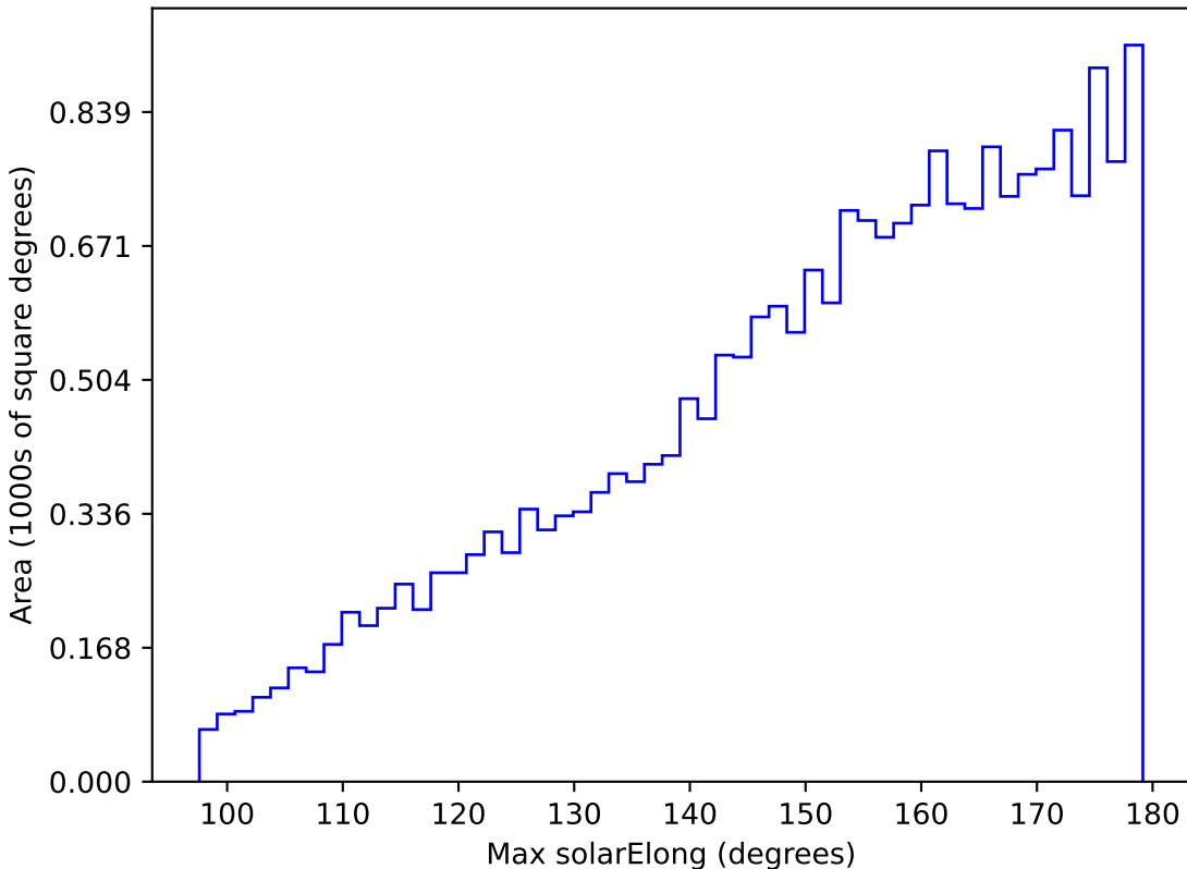
telescope_jerk_v3.5_10yrs All sky y band: Max solarElong
