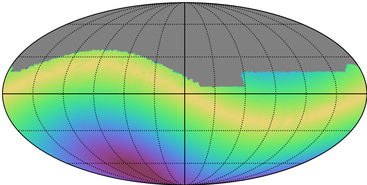
telescope_jerk_v3.5_10yrs All sky r band: Max solarElong
