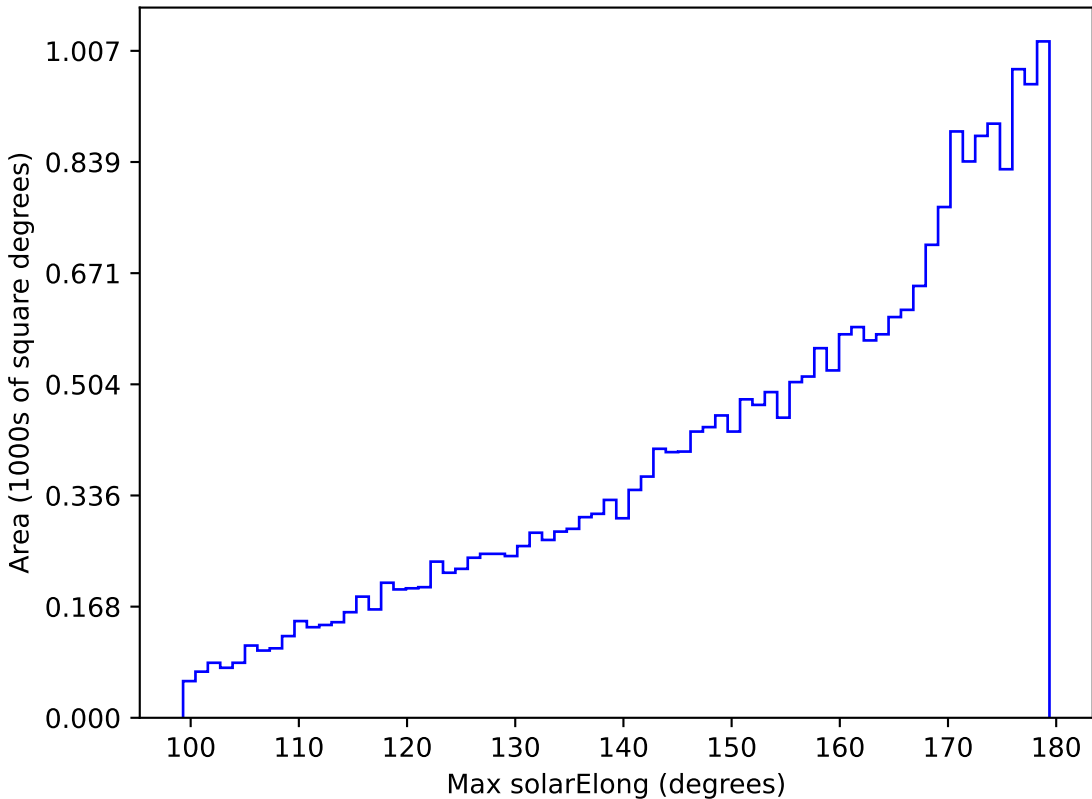
telescope_jerk_v3.5_10yrs All sky r band: Max solarElong
