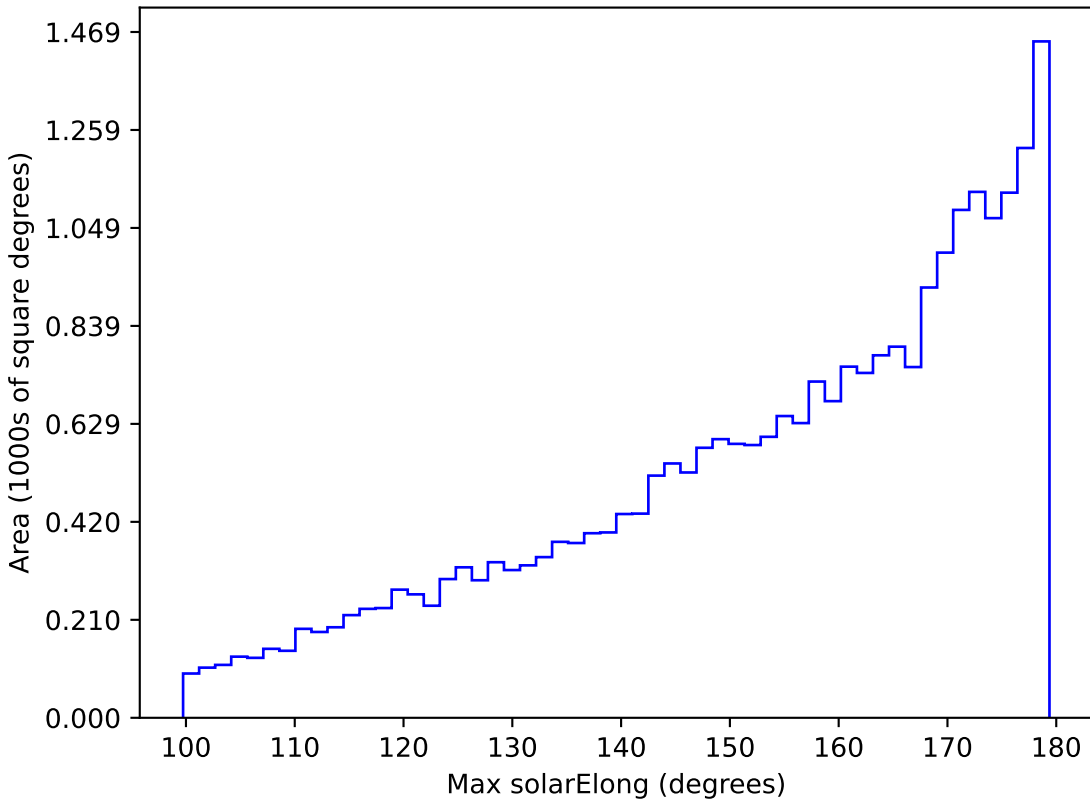
telescope_jerk_v3.5_10yrs All sky i band: Max solarElong
