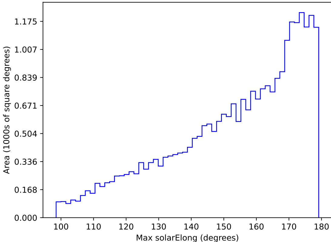
telescope_jerk_v3.5_10yrs All sky g band: Max solarElong
