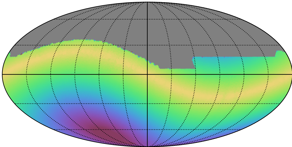
telescope_jerk_v3.5_10yrs All sky all bands: Max solarElong
