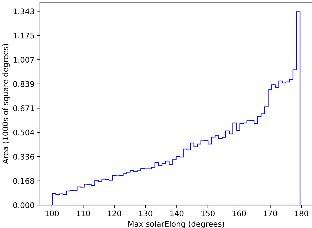
telescope_jerk_v3.5_10yrs All sky all bands: Max solarElong
