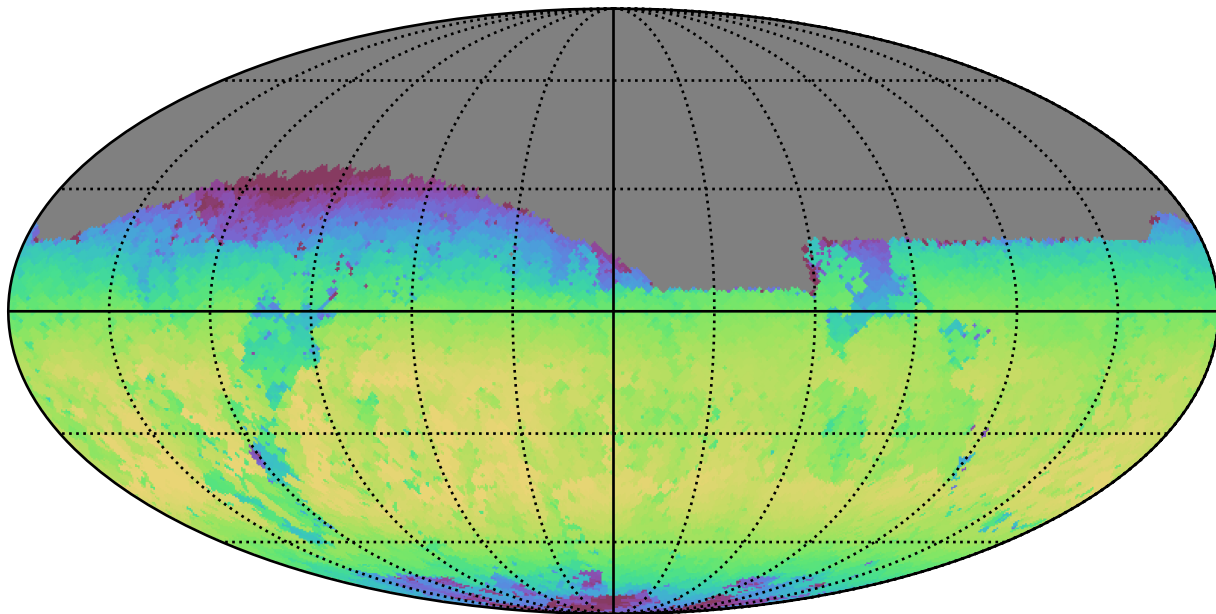
telescope_jerk_v3.5_10yrs Yr 1 z band: Max skyBrightness
