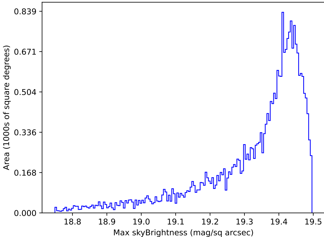
telescope_jerk_v3.5_10yrs Yr 1 z band: Max skyBrightness
