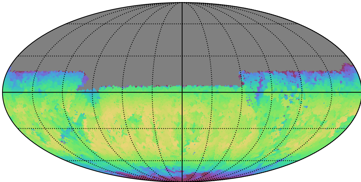
telescope_jerk_v3.5_10yrs Yr 1 y band: Max skyBrightness
