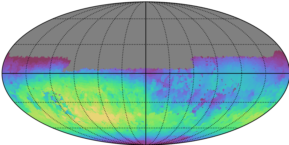
telescope_jerk_v3.5_10yrs Yr 1 u band: Max skyBrightness
