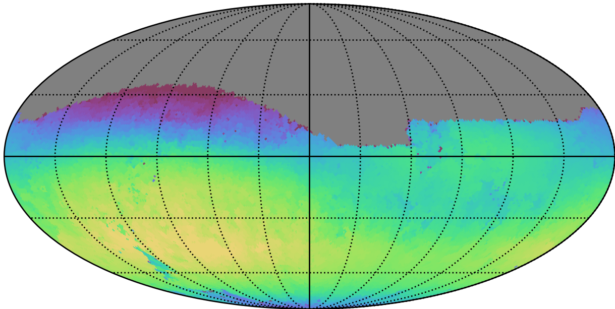
telescope_jerk_v3.5_10yrs Yr 1 r band: Max skyBrightness
