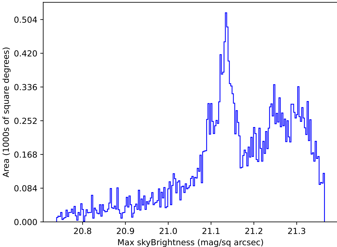
telescope_jerk_v3.5_10yrs Yr 1 r band: Max skyBrightness
