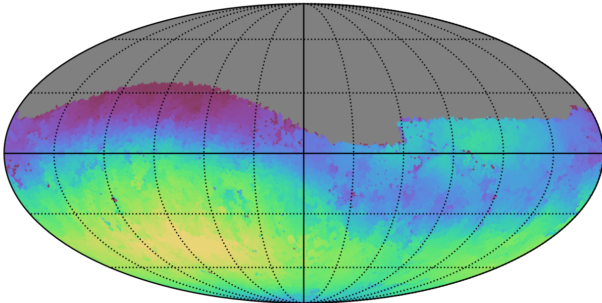
telescope_jerk_v3.5_10yrs Yr 1 g band: Max skyBrightness
