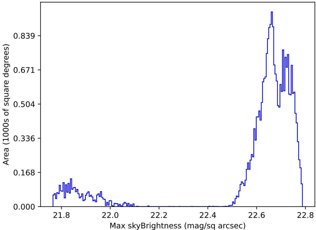
telescope_jerk_v3.5_10yrs Yr 1 all bands: Max skyBrightness
