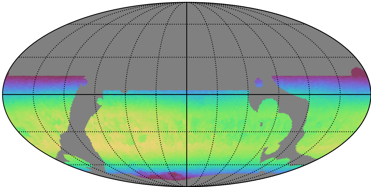
telescope_jerk_v3.5_10yrs WFD z band: Max skyBrightness
