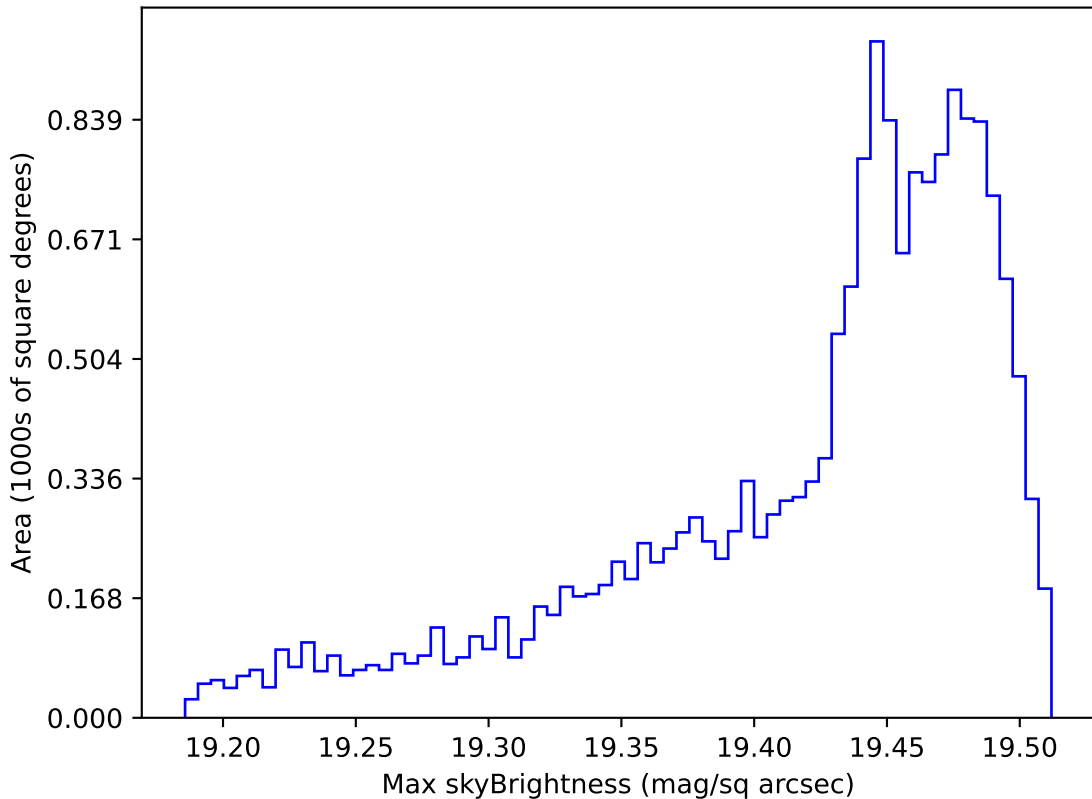
telescope_jerk_v3.5_10yrs WFD z band: Max skyBrightness
