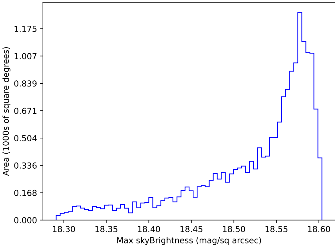
telescope_jerk_v3.5_10yrs WFD y band: Max skyBrightness
