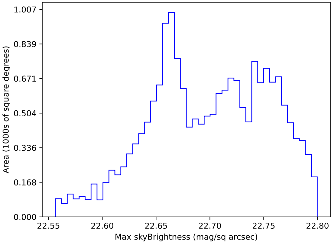
telescope_jerk_v3.5_10yrs WFD u band: Max skyBrightness
