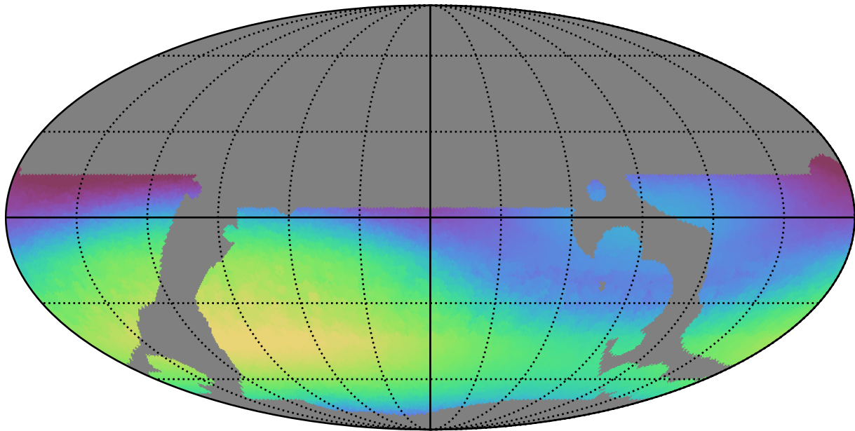
telescope_jerk_v3.5_10yrs WFD r band: Max skyBrightness
