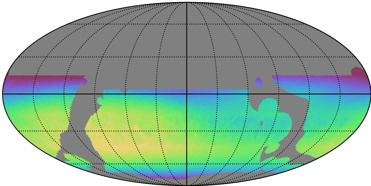
telescope_jerk_v3.5_10yrs WFD i band: Max skyBrightness
