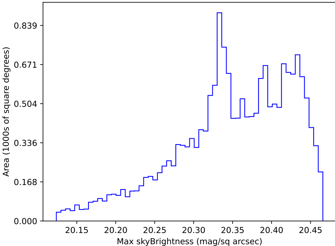
telescope_jerk_v3.5_10yrs WFD i band: Max skyBrightness
