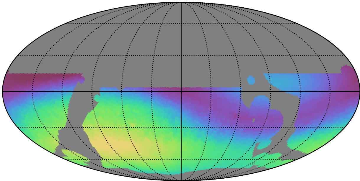
telescope_jerk_v3.5_10yrs WFD g band: Max skyBrightness
