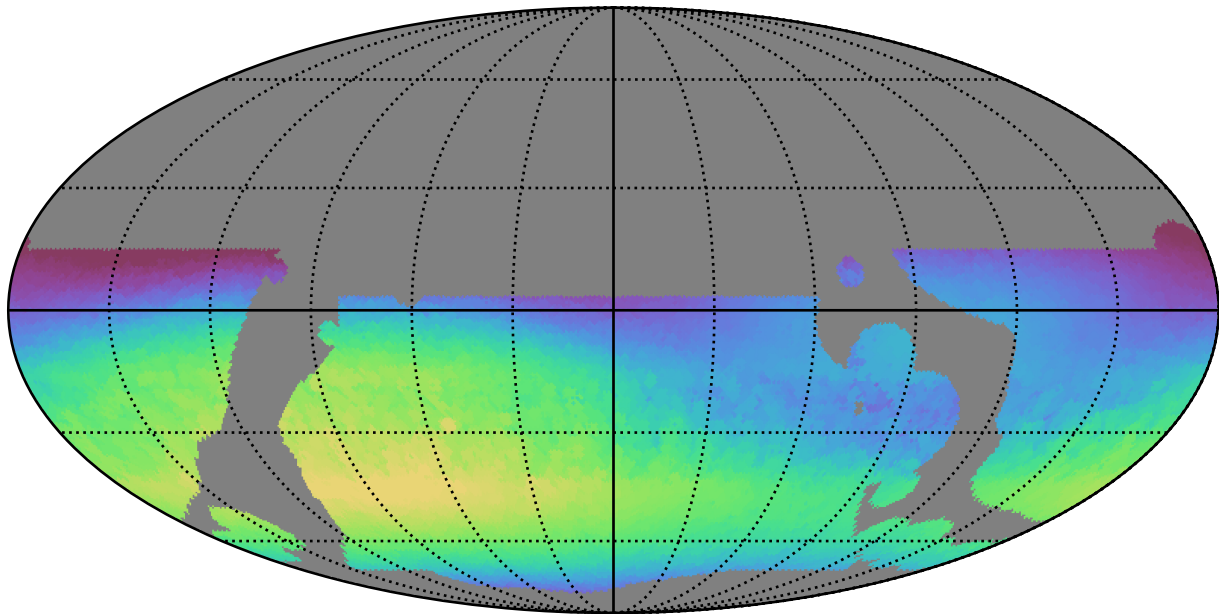
telescope_jerk_v3.5_10yrs WFD all bands: Max skyBrightness
